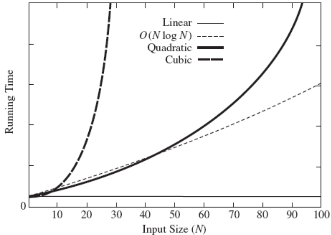
Figure 2.3 Plot ( N vs. time) of various algorithms
